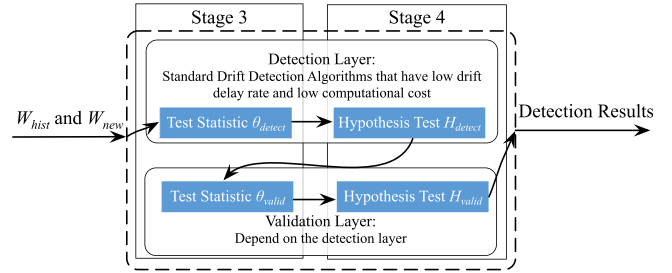
Fig. 10. Hierarchical multiple hypothesis test drift detection.
